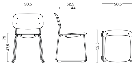
SOFT EDGE 55 SLED | SEAT UPHOLSTERY WIDTH 50,5 CM DEPTH 52,5 CM HEIGHT 79 CM SEAT HEIGHT 47,5 CM SEAT DEPTH 44 CM
